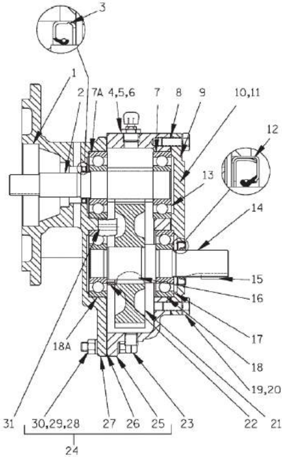
Figure 2. 44161-014 Gearbox Assembly
